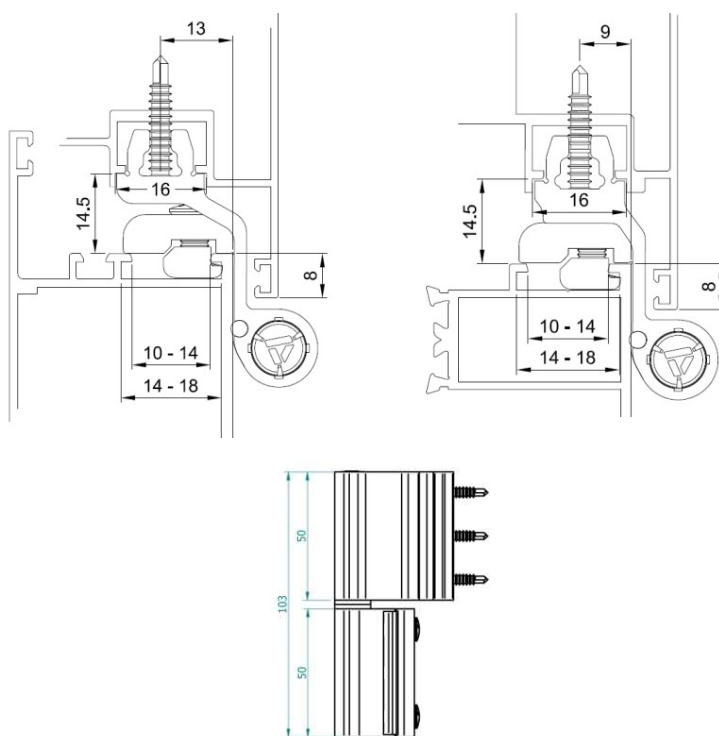
DIMENSIONS (mm)
